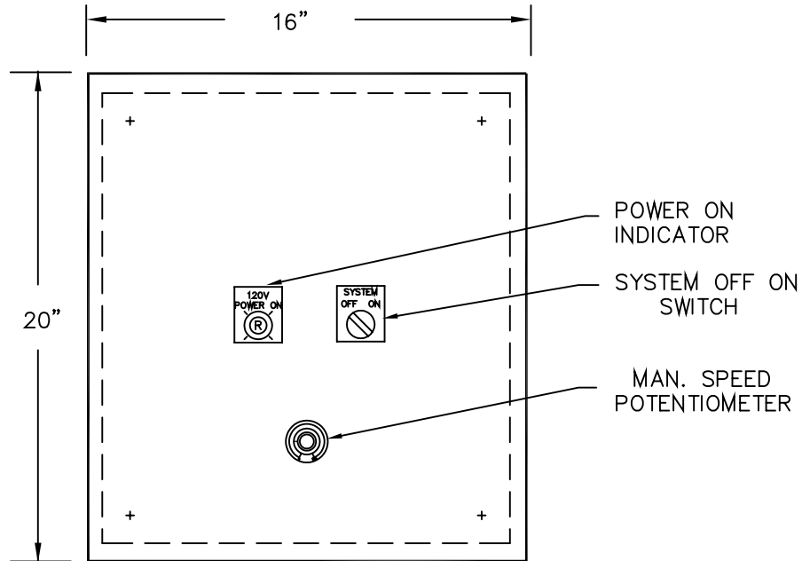
WALL MOUNT ENCLOSURE DIM.: 20" x 16" x 6"
