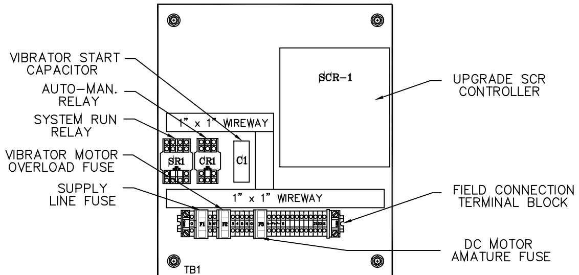
PANEL LAYOUT V.S.I. P/N: VS-DC UPGRADE
